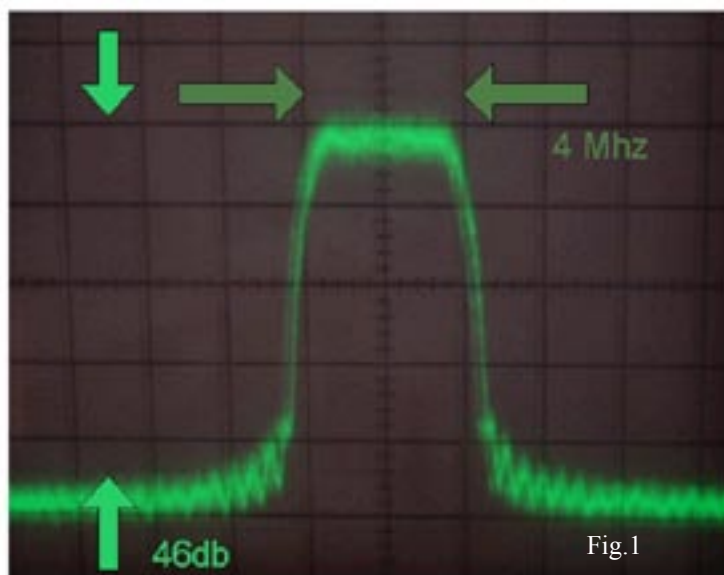
QPSK at FEC 7/8 3.5Msymbols/s
