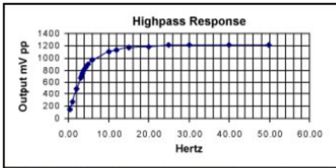
Figure 4. Frequency response of AC-coupled video connection with 220 \mu F capacitor.
