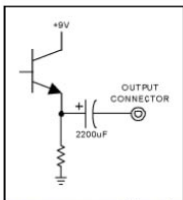
Figure 3. NPN emitter follower driving a load.
