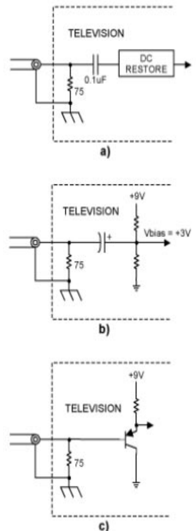
Figure 6. a) Modern TV input stage, b) polarized capacitor c) PNP emitter follower in input stage.
